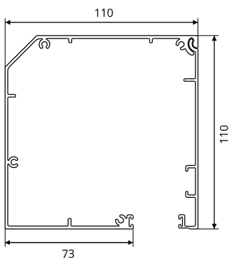
CASSETTE 110 | KASETA 110 CAISSON 110 | KASSETTE 110
