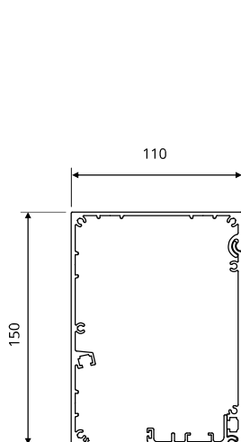
CASSETTE 110 COMPACT | KASETA 110 COMPACT CAISSON 110 COMPACT | KASSETTE 110 COMPACT
